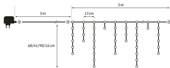
In & Outdoor | Connect Icicle 100 LED warmwhite | 3 x 0,9 m white cable | ⚡ 3 m | 31V 6W 20 strings | 12x connectable Art. DKL-242-01 | CHF 59.00
