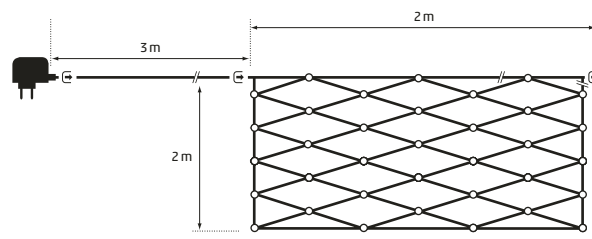
In & Outdoor | Connect Net 160 LED warmwhite | 2 x 2 m green cable | ⚡ 3 m | 31V 6W 7x connectable Art. DKL-266-01 | CHF 79.00
