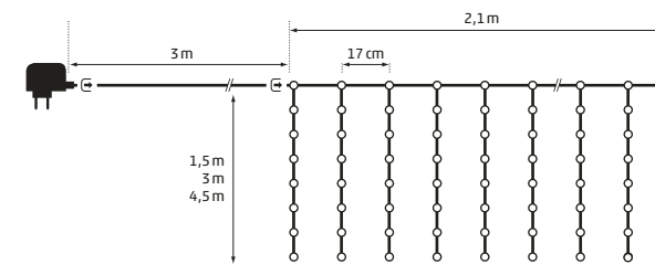
In & Outdoor | Connect Curtain 140 LED warmwhite | 2,1 x 1,5 m green cable | ⚡ 3 m | 31V 6W 14 strings | 8x connectable Art. DKL-261-01 | CHF 79.00
